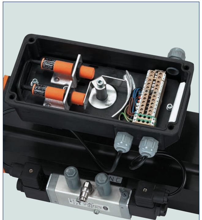
Pneumatic quarter turn actuator (double acting) with switch box NSK (Size II). Integrated proximity switches. Support acc. to VDI/VDE 3845. Compound coil pilot solenoid valve.
